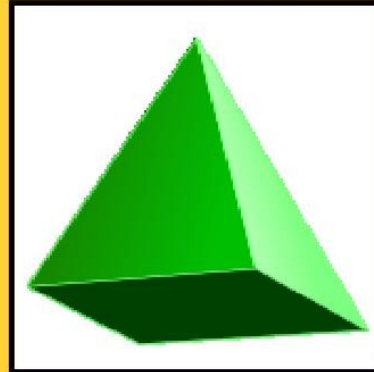
Square-based pyramid
