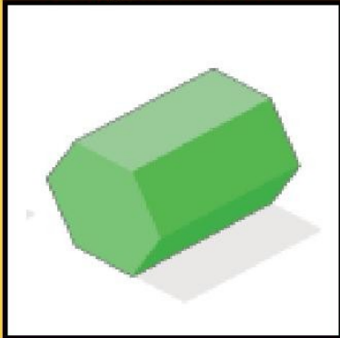
Hexagonal Prism
