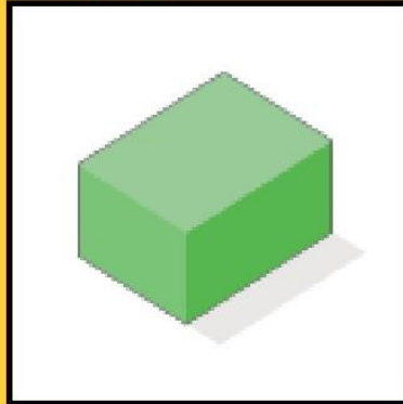
Cuboid
