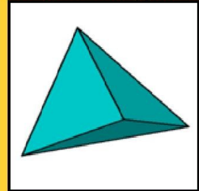
Triangular-base pyramid
