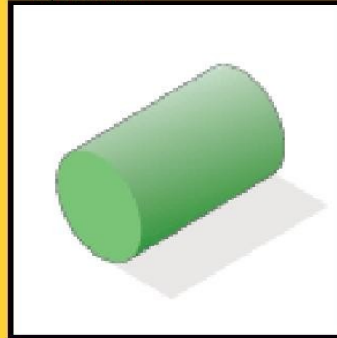
Cylinder
