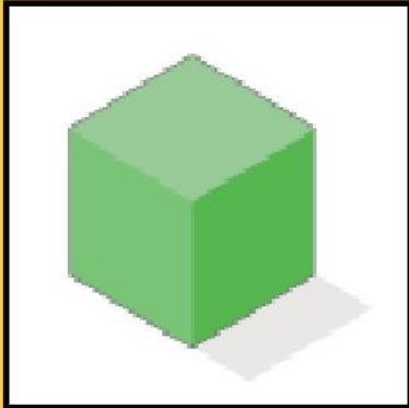
Cube
